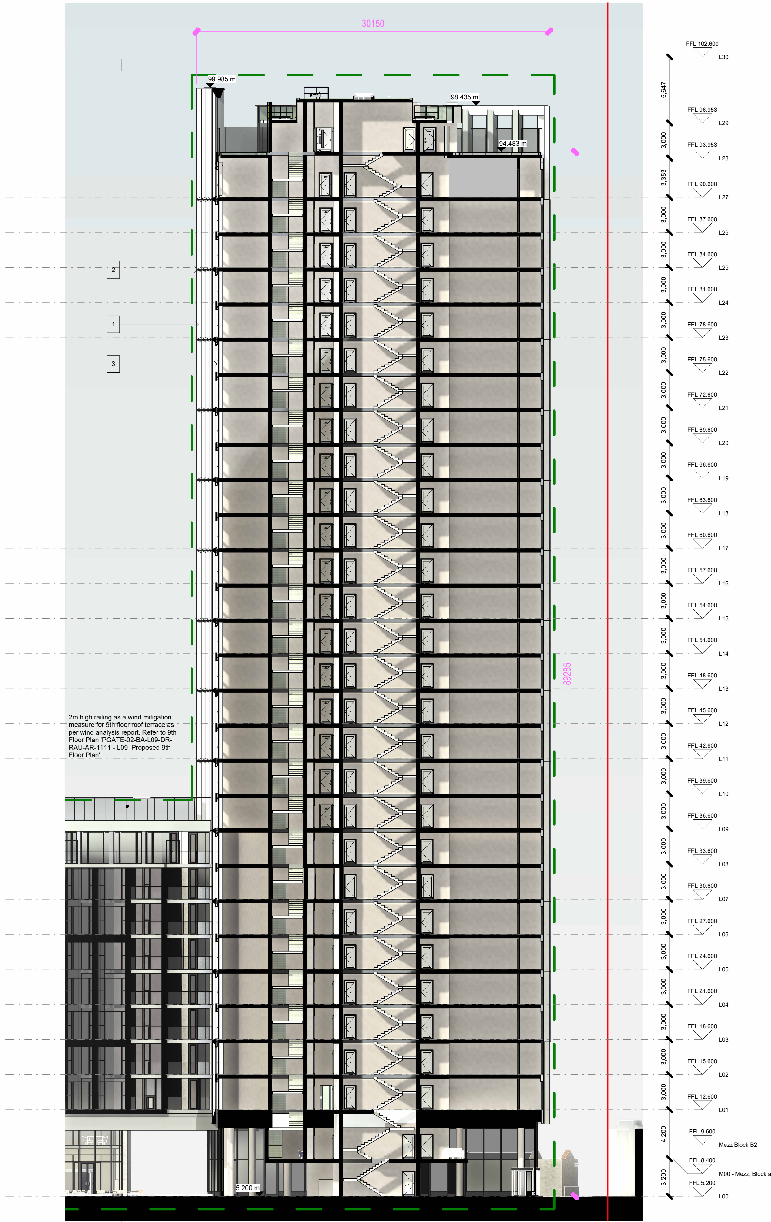
Proposed Section CC 1 : 200
