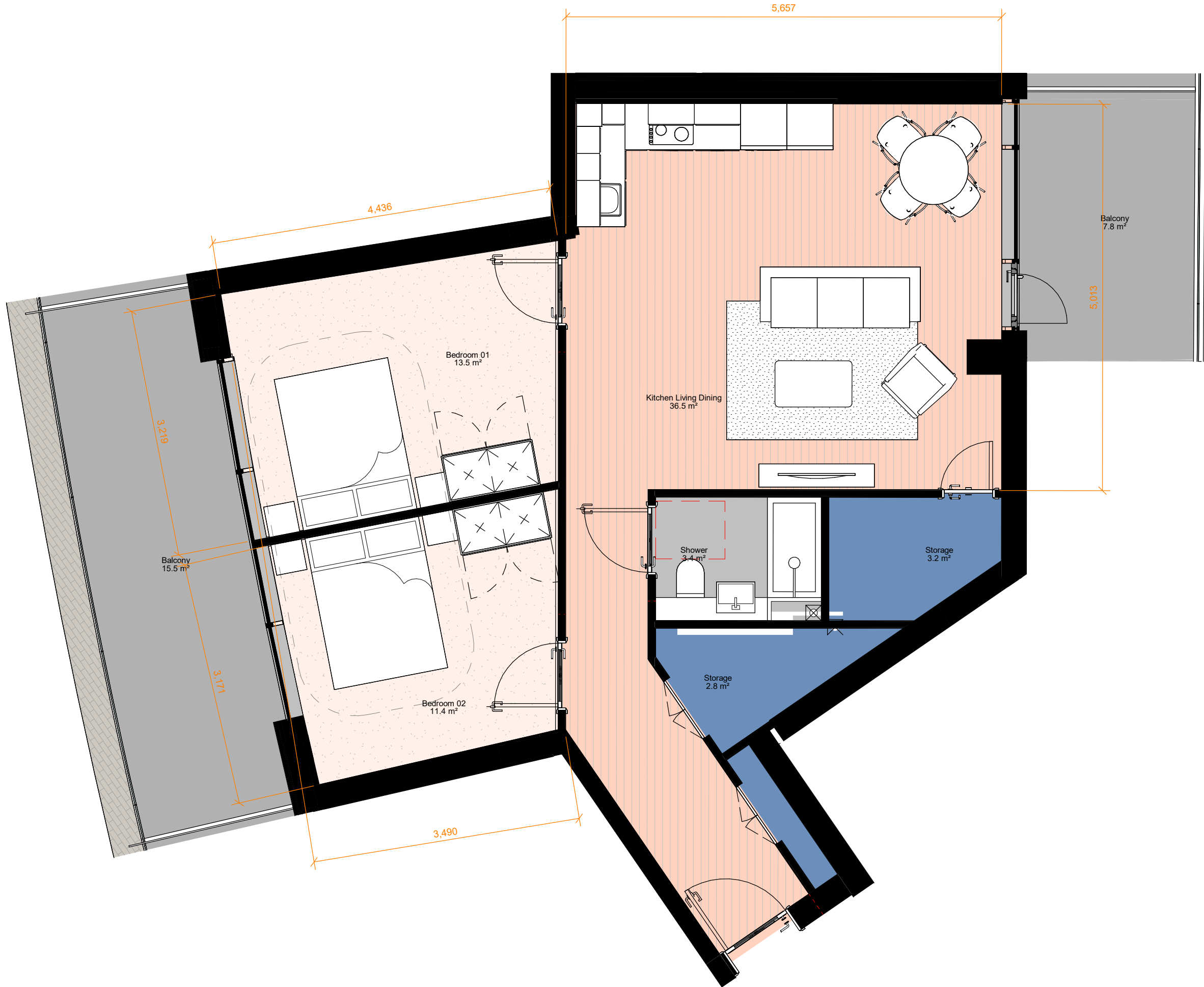
Unit Type - B208 - Two Bedroom 1 : 50
